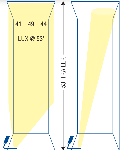
LED Versa Light® illuminates the entire trailer
